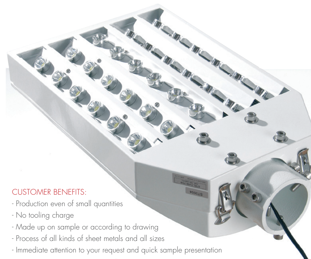
STREET 02 ■ Stainless Steel SUS430, powder-coated. Electrification provided by the customer. 48 cm x 28 cm x 11 cm
